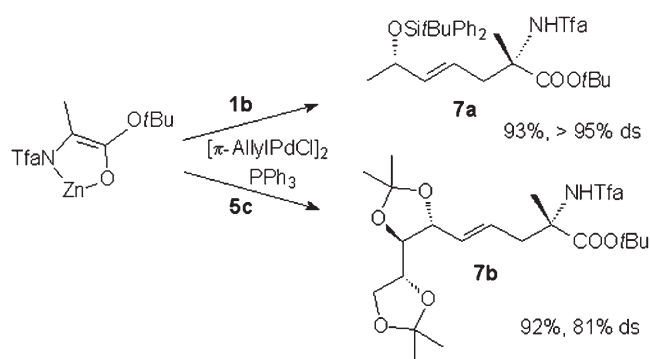
Scheme 6. Synthesis of \alpha -allylated amino acids.
